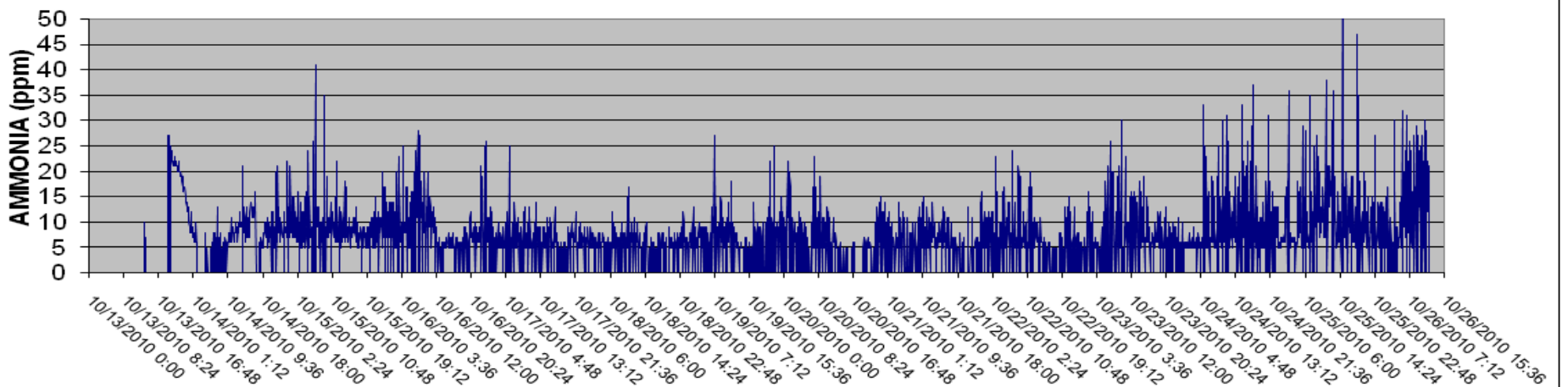
Poultry House Ammonia Concentrations, Ventilation Scheme 2
